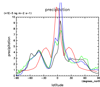
Figure 101: Rain at May by DCPAM (red), NCEP (green), ECMWF (blue), and GPCP (black)
