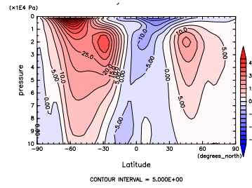
Figure 238: U at Aug. by DCPAM
