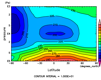
Figure 706: T at Aug. by DCPAM
