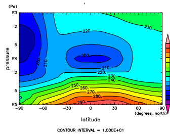
Figure 707: T at Aug. by NCEP
