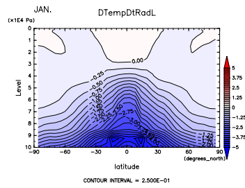
Figure 517: (\partial T/\partial t)_{LW} at Jan. by DCPAM
