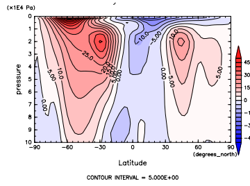
Figure 235: U at Jul. by DCPAM
