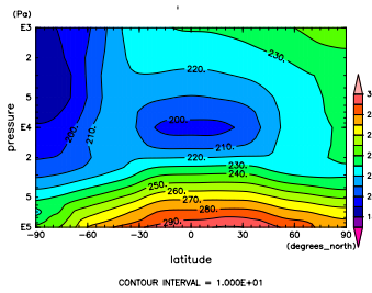
Figure 704: T at Jul. by NCEP
