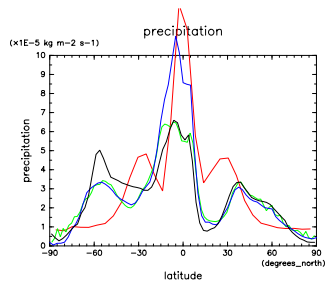
Figure 98: Rain at Feb. by DCPAM (red), NCEP (green), ECMWF (blue), and GPCP (black)
