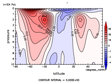
Figure 236: U at Jul. by NCEP
