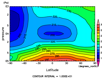
Figure 703: T at Jul. by DCPAM
