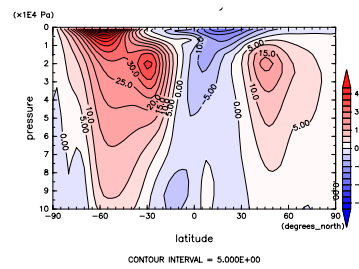
Figure 239: U at Aug. by NCEP
