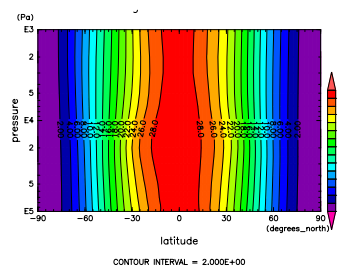
Figure 602: ANGMOM at Sep. by NCEP by Figure 605: ANGMOM at Oct. by NCEP
