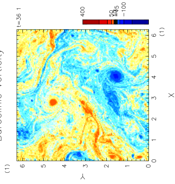
Baroclinic Vorticity
